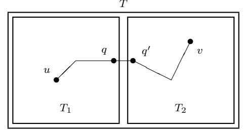
Fig. 2 Finding \pi_3 = \pi(u, v) .
