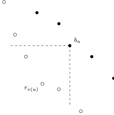
Fig. 3 Computing r_{v(u)} for b_u .
