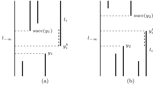
Fig. 6 (a) l_{-\infty} is visible from y_i^b . (b) l_{-\infty} is visible from y_i^t . The dashed part of l_i is now on the left envelope.
