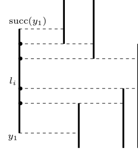
Fig. 7 If l_i is deleted, the part hidden by l_i newly appears on the left envelope. The four dots indicate the tuples from B_i , which means that from l_i , the four top or bottom points corresponding to the circles are visible.
