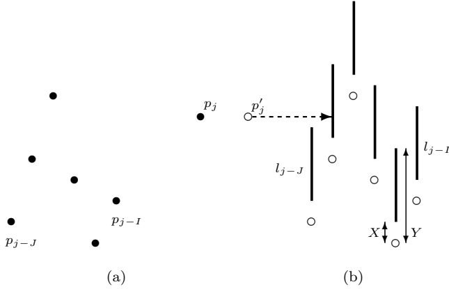
Fig. 1 (a) Point p_j and points p_{j-J}, \dots, p_{j-I} are shown. (b) Segments l_{j-J}, \dots, l_{j-I} are depicted and the ray starting at p'_j hits one of the segments, which is l_{\lambda_j} . The circles indicate where the points were.
