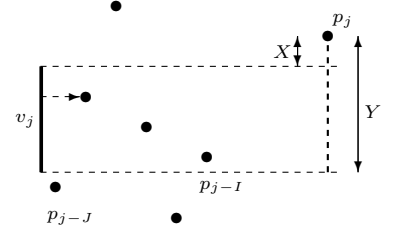
Fig. 13 Point p_j and points p_{j-J}, \dots, p_{j-I} are shown. The segment v_j is moving rightward and hits one of the points, which is p_{\lambda_j} .
