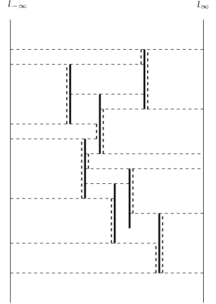
Fig. 2 The right and left envelopes of seven segments of the same length. The right envelope consists of five fragments, and the left envelope consists of six fragments. Fragments of the right (resp., left) envelope are shown dashed lines on the right-hand (resp., left-hand) side of each segment.
