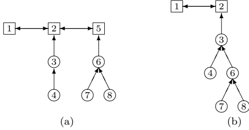
Fig. 12 (a) The data structure for D = (1, 2, 3, 4, 5, 6, 7, 8) of Fig. 10, which has two blocks. The blue integers ( \square ) are stored in a doubly linked list and the red integers ( \circ ) are stored into sets (or rooted trees). Each root points to its current blue neighbor. (b) The data structure after deleting 5 is shown. The trees with root 3 and with root 6 are merged into one.
