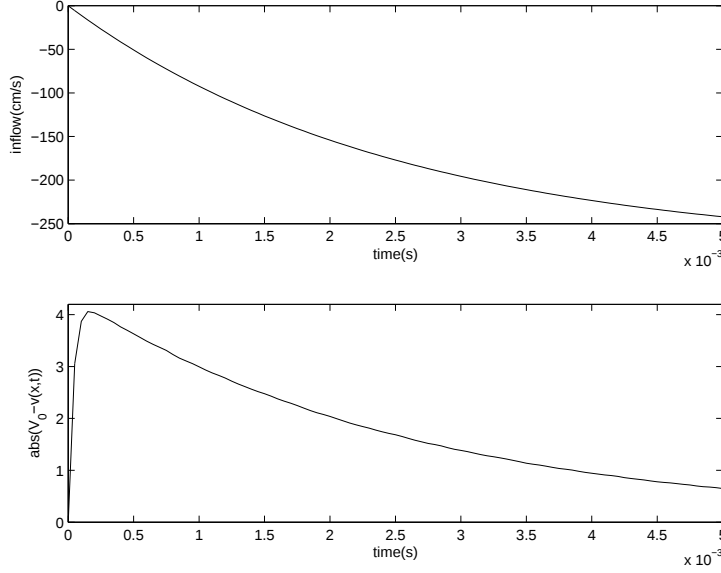
Fig. 7. The top panel represents the y-component V_0(t) of the desired inflow, and the bottom panel is the absolute error of the y-component of the calculated velocity v(\mathbf{x}, t) from the desired velocity V_0(t) at one specified point \mathbf{x} , i.e., |V_0(t) - v(\mathbf{x}, t)| .
