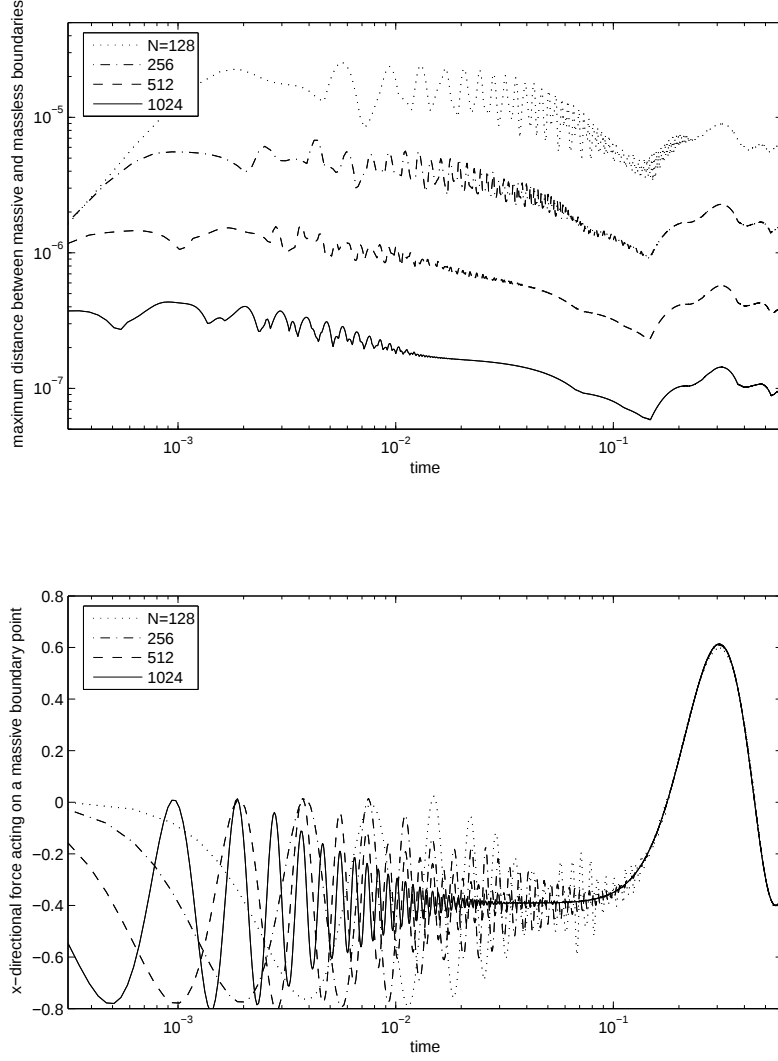
Fig. 4. The maximum amplitude \|\mathbf{X} - \mathbf{Y}\|_\infty of the oscillation (distance between the two shells) and the x-directional force -\mathbf{F}_K acting on a massive boundary point (‘*’ in Fig. 2) are plotted in time for each N . As N gets bigger, the computation gets refined and K increases. As the refinement goes on, the maximum distance of the two shells decreases (top panel), and the force acting on the chosen point converges (bottom panel).
