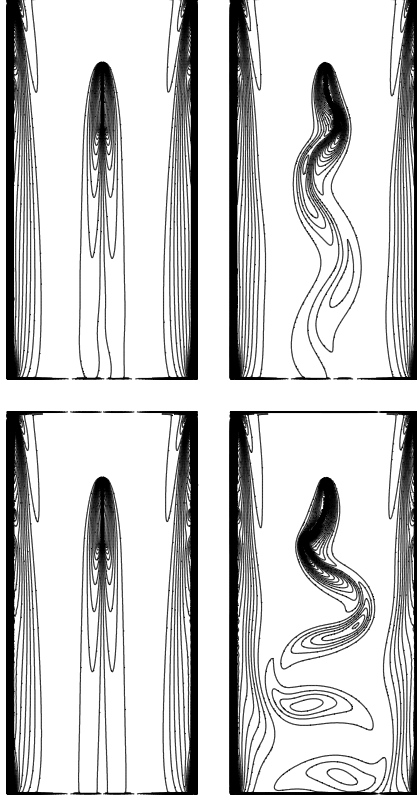
Fig. 9. Motion of two filaments with different mass densities: 10^{-5}\text{g/cm} (left panels) and 4 \times 10^{-4}\text{g/cm} (right panels). The vorticity contours are drawn at two different times: 0.06s (top) and 0.18s (bottom).
