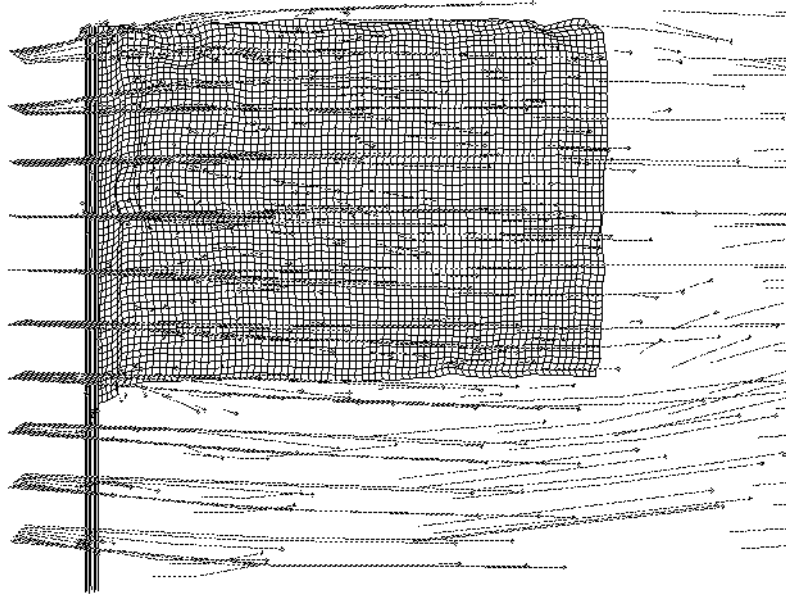
Fig. 20. Motion of the massless flag. Even though all other conditions are same as in Fig. 18 top, the massless flag neither flaps nor sags. See also Fig. 21.
