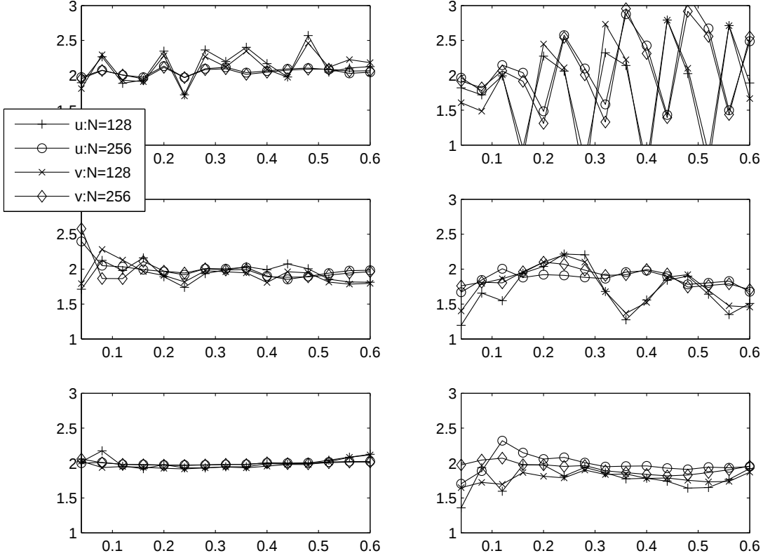
Fig. 3. Convergence rates of velocity field (u, v) in time in three different cases: massless (first row), non-tapered constant massive (second row), and tapered massive (third row). The left and right columns have two different fluid viscosity 0.005 and 0.0005, respectively. The left column shows that the convergence rates are roughly equal to 2 regardless of the mass of the fibers. When the Reynolds number is too high (right column), the convergence rate drops and recovers again to almost 2 when the grid resolution becomes fine enough.
