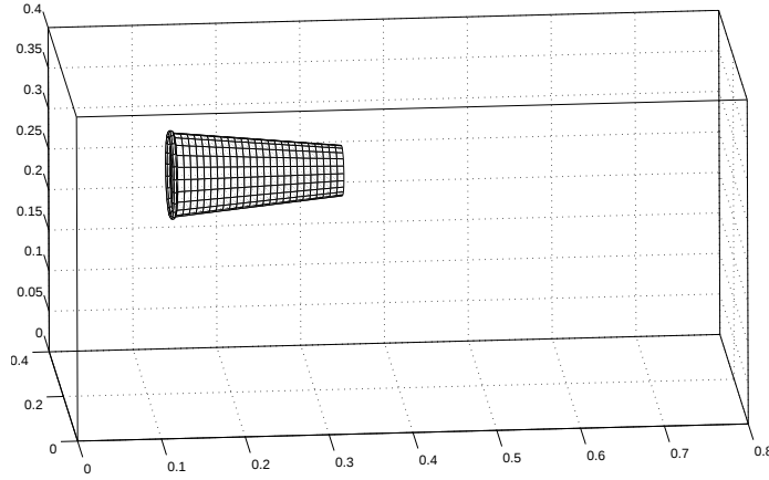
Fig. 12. Initial configuration of windsock and computational domain which is a box 0.8 \times 0.4 \times 0.4 \text{ m}^3 . The left end of the windsock is attached to a ring which is fixed in the domain. Wind is driven from left to right by prescribing inflow velocity at the left face of the domain.
