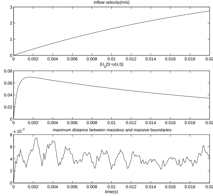
Fig. 13. Errors in the windsock simulation. The top graph represents the x-component U_0(t) of the desired inflow, and the middle graph is the absolute error of x-component of the induced velocity u(\mathbf{x}, t) from the desired one U_0(t) at one specified point \mathbf{x} , i.e. |U_0(t) - u(\mathbf{x}, t)| . The maximum distance (in units of meshwidth) between two boundaries is shown in the bottom graph. Note that the maximum distance between the massive and massless boundaries is always less than 8 \times 10^{-5} meshwidths.
