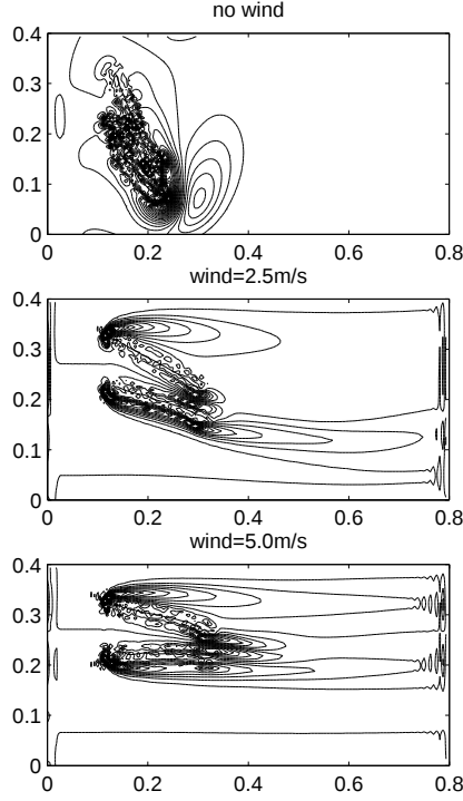
Fig. 14. Three different cases of a windsock are compared. Vorticity contours in a vertical plane that bisects the windsock are plotted. The top frame has no wind and the windsock falls down. In the case of a small wind speed (middle), the windsock finds an equilibrium angle that depends on the wind speed. The bottom frame has a large wind speed which straightens the windsock.
