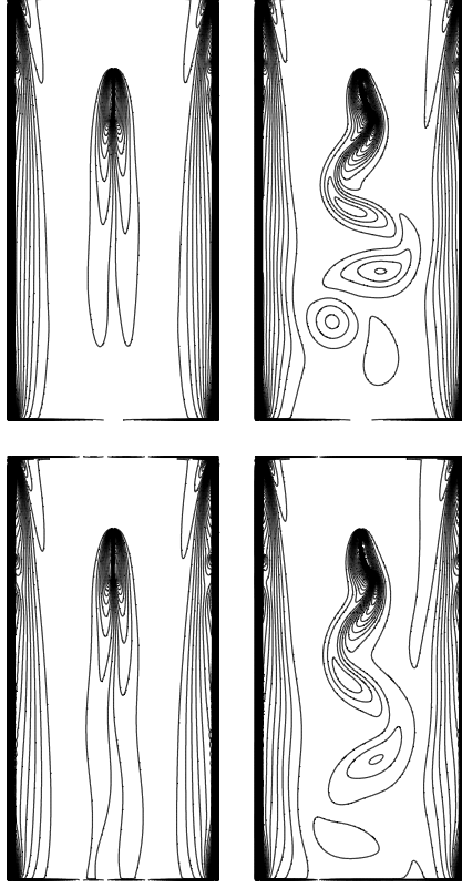
Fig. 11. Motion of a filament with all the same circumstances except the initial conditions (see figure 8): a small perturbation (left) and a large one (right). The vorticity contours are drawn at two different times: 0.06s (top) and 0.18s (bottom).
