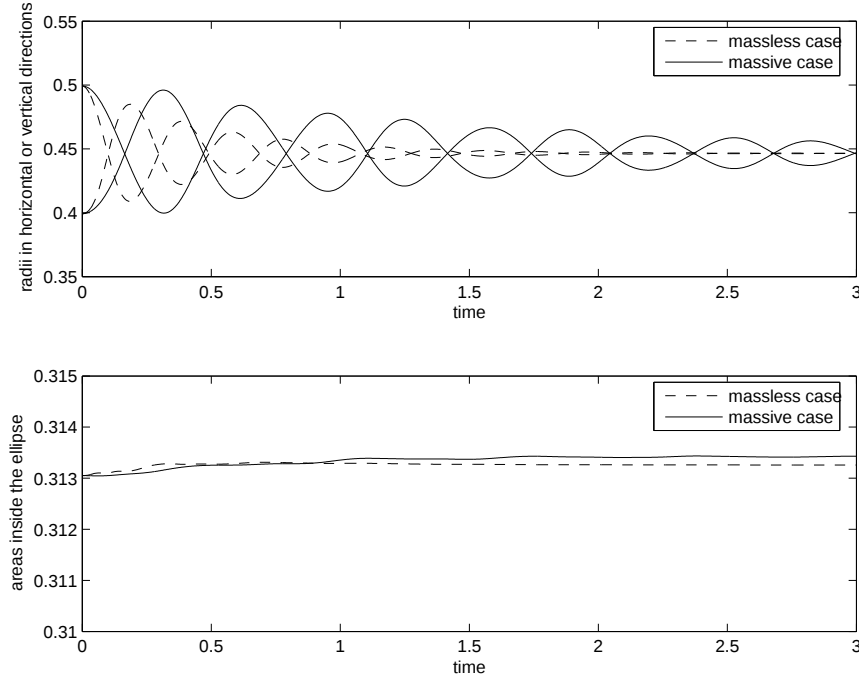
Fig. 5. The influence of boundary mass on the behavior of an immersed elastic boundary in the form of a simple closed curve in a two-dimensional fluid. The curve is initially elliptical, and the horizontal and vertical radii are plotted as functions of time. Both cases show a damped oscillation as the boundary approaches a circular shape, but the massive boundary oscillation has a lower frequency and is sustained longer than that of the massless boundary. The overall downward trend is a form of numerical error (see text) that is somewhat exaggerated here by the vertical scale of the plot.
