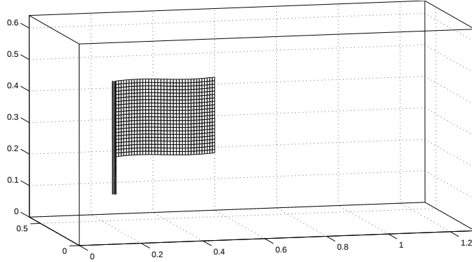
Fig. 17. Initial configuration of a flag and the computational domain which is a box 1.28 \times 0.64 \times 0.64 \text{m}^3 . The left end part of the flag is attached with the flagpole which is fixed in the domain. The flow of the wind is from left to right.
