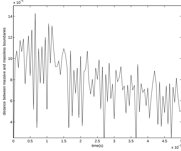
Fig. 6. The maximum distance in units of meshwidth between the massless and massive boundaries as a function of time. The maximum distance between two boundaries stays below 1.5 \times 10^{-4} meshwidth here and even after the time shown in this graph.
