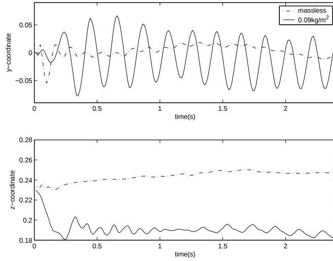
Fig. 21. Comparison of the motions of two flags with and without mass. Trajectories of the (y, z) coordinates of the lower downstream corners of the two flags are plotted, with the solid lines corresponding to the flag with mass, and the broken lines corresponding to the flag without mass. The massive flag flaps (top panel) and sags (bottom panel) but the massless flag does neither.
