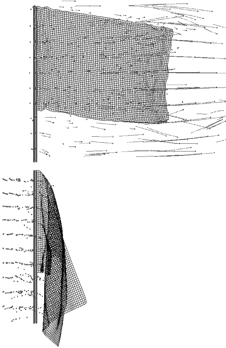
Fig. 18. A large enough windspeed (top) helps the flag overcome the gravity and sustain a flapping motion. We can see the flag still sagging slightly. In the case of no wind (bottom), the flag falls down and stops moving. Note the folds which are a consequence of the (small) bending rigidity of the flag. (time=1.2s)
