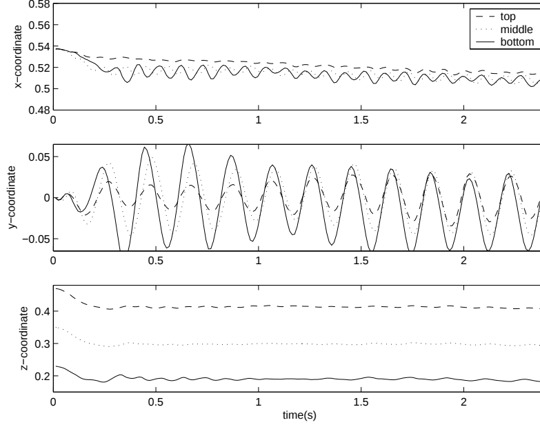
Fig. 19. Cartesian coordinates of the positions of three different material points on the downstream edge of the flag. Three points are chosen at the top, middle, and bottom of the downstream edge. The x-axis is in the direction of the wind, the y-axis is perpendicular to the flag and the wind direction, and the z-axis is vertical. We can see from the middle panel that the flag is flapping, and, from the bottom panel, that the flag sags a little at the beginning of the computation and then stops sagging. Note (middle panel) that the flapping motions of top and bottom of the flag are out of phase, i.e. the bottom part runs ahead of the top part. Also the amplitude of the flapping motion is much greater at the bottom of the free edge than at the top.
