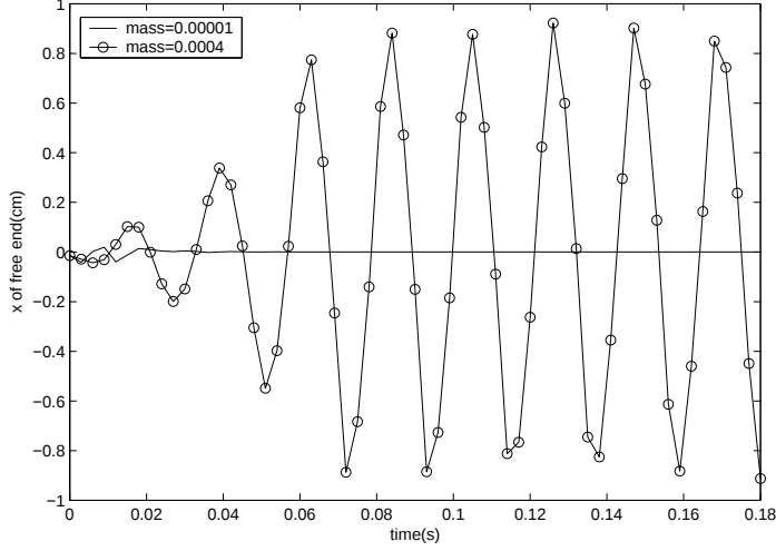
Fig. 8. The x -coordinate of the free ends of two filaments are plotted as functions of time. The sustained flapping motion is observed only in the case of a filament with enough mass.
