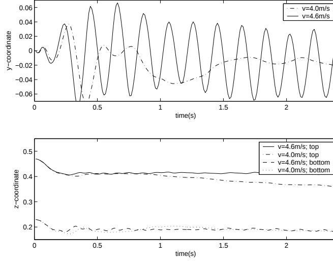
Fig. 23. Comparison of flag motions with low and high wind speed. The figure shows (y, z) -coordinates of the positions of selected points of the downstream edge of the two flags as functions of time: the inflow velocities are 4.0m/s and 4.6m/s. From the upper panel it is clear that the flag in the slower wind is not flapping although its position is not perfectly steady either. The heights of the downstream-bottom point of both flags is almost same, but the downstream-top point of the slower wind case is lower than that of the faster wind case. This implies that the downstream edge of the flag in the slower wind is bent, which is a typical phenomenon when a flag does not flap, see also Fig. 22.
