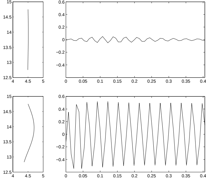
Fig. 10. The left two pictures show the initial configurations of a filament in the shape of a sine curve with two different amplitudes: 0.01cm (left-top) and 0.2cm (left-bottom). The x -coordinate of the free ends of the two filaments are plotted as functions of time in the right two panels. While the case with a small initial perturbation almost stops flapping (top), the large initial perturbation case quickly settles into a sustained oscillation with a larger amplitude than that prescribed initially (bottom).
