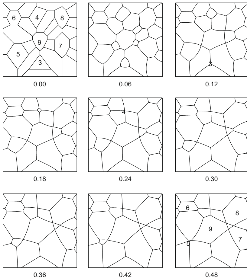
Fig. 11. The motion of a general foam at some chosen times. The cells of less than six edges shrink and eventually disappear, whereas those with more than six edges grow. This results in the coarsening of the foam. The number below each frame is the time to which that frame corresponds. In the frame showing the initial configuration, selected cells are numbered according to their number of edges. The disappearance of cell #3 occurs at t = 0.12 , that of cell #4 occurs at t = 0.24 , and that of cell #5 occurs at t = 0.48 .
