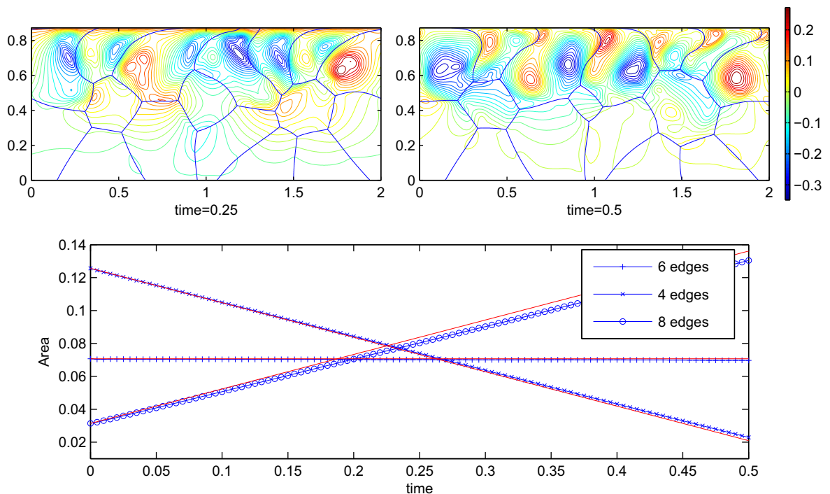
Fig. 10. Foam driven by oscillatory shear. Target points near the upper boundary slide left and right in an oscillatory motion with frequency 10\pi and amplitude 0.25. Target points on the lower boundary are held fixed. There are no target points on the left or right boundary, so the motion is periodic in x . The configuration and motion of the foam are shown at t = 0.25 (upper left) and t = 0.5 (upper right), with the velocity field plotted in terms of streamlines. The areas of the three central cells are plotted as functions of time in the lower panel, where the predictions of the von Neumann relation are shown for comparison as solid lines. Even though the foam is far from equilibrium, the von Neumann relation is well satisfied.
