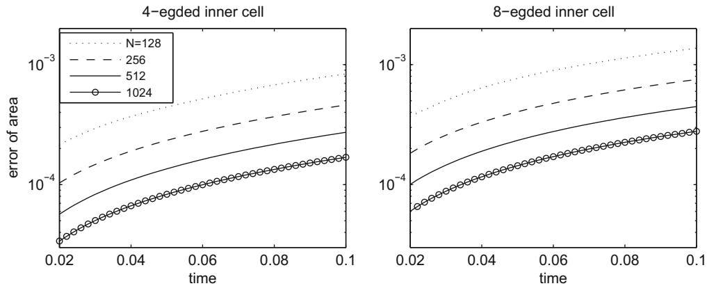
Fig. 7. The errors of area in comparison to that predicted by the von Neumann relation are plotted as functions of time on a logarithmic vertical scale for each of the cases N = 128, 256, 512 , and 1024 . The left panel is for a 4-sided cell and the right panel is for an 8-sided cell. Note the decrease of the error as N increases.
