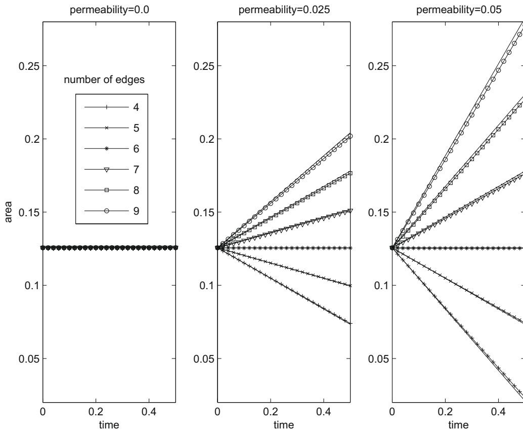
Fig. 5. The change of the inner cell area with time. The number of edges varies from n=4 to n=9 , and the permeability parameters are M=0 (left), M=0.025 (middle), and M=0.05 (right). The changes of the inner cell areas are linear and almost follow the von Neumann relation, which is represented by the solid lines.
