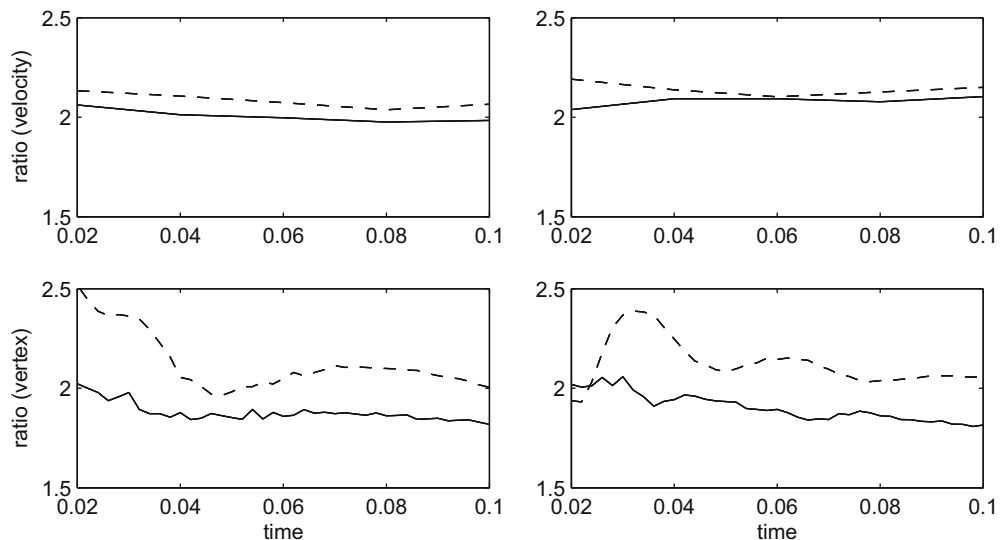
Fig. 8. Convergence ratios of the computed velocity field \mathbf{u}(\mathbf{x}, t) of the fluid (top) and the position (x_N^i, y_N^i) of vertices (bottom). The convergence ratios (defined in the text) are plotted as functions of time for two different cases: 4-sided inner cell (left) and 8-sided inner cell (right). In each panel, the dashed line is the convergence ratio obtained using the grids N = 128, 256 , and 512 , and the solid line is the rate obtained with N = 256, 512 , and 1024 . The convergence ratio is near 2 (first-order accuracy).
