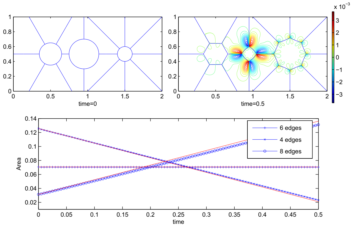
Fig. 9. The motion of a foam at t = 0 (top-left) and t = 0.5 (top-right) with streamlines depicting the velocity field, and the areas of the three inner cells plotted as functions of time (bottom). The areas follow the von Neumann relation (solid lines with no symbols).
